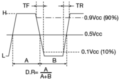
Figure 3) HCMOS Output Wave Form
