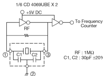
Figure 2) ZTT□.□□MG Test Circuit
